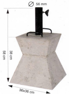
RESORT STAND Size M/NW. 63 Kgs.
