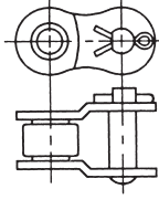
OFFSET LINK contour side bar
