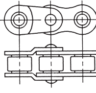
TWO PITCH OFFSET LINK
