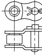
OFFSET LINK contour side bar
