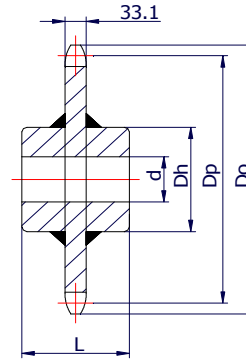
Welded construction CW type
