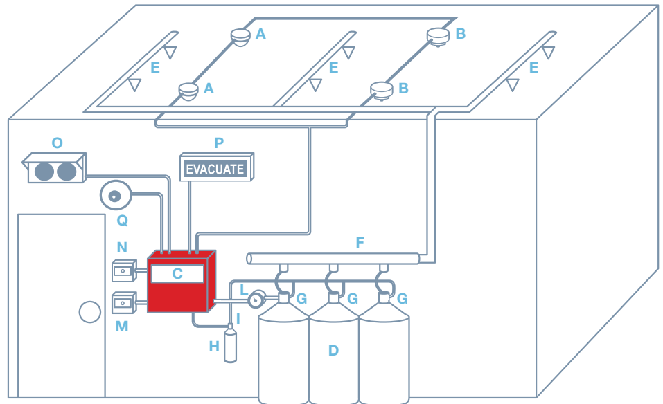
Application diagram
