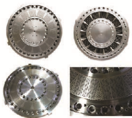
Die plates for PP, PE, EVA
