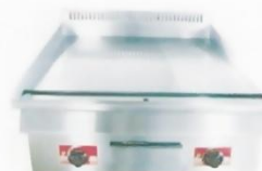
Gas Griddle (Flat Plate) Model : ET-TGG-75 W820xD780xH380mm Power:54,560BTU/hr N/W:66kg
