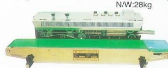
Solid-ink Printing Sealer Model : ET-FRD-1000W Size : 1060x470x380 mm Power : 750W Voltage : 220V/50Hz Sealing speed : 0~18 m/min Sealing Width : 6-15 mm Temperature Range : 0-300 °C
