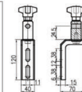
Stainless steel bracket adjustment set
