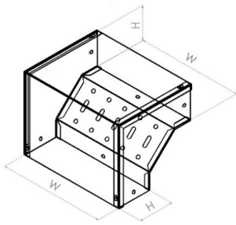
OUTSIDE VERTICAL
