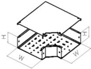
HORIZONTAL ELBOW 90
